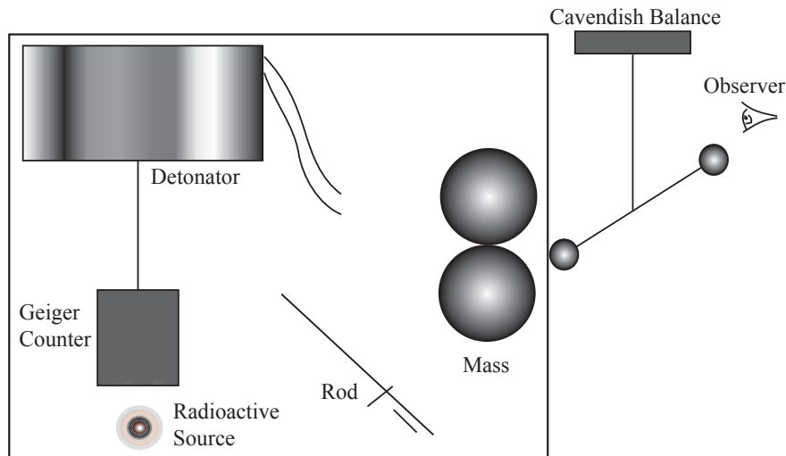
FIG. 5.2. Unruh's Schrödinger-Cavendish experiment: final state
