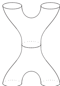
FIG. 5.3. Interactions between strings take place by (local) joining and splitting, i.e. when two points of the strings touch—xy-pic code used with the kind permission of Aaron Lauda.
