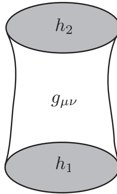
FIG. 5.5. Representation of the gravitational path integral as a gravitational propagator from an initial 3-geometry h_1 to a final 3-geometry h_2 , interpolated by the 4-geometry g_{\mu\nu}
