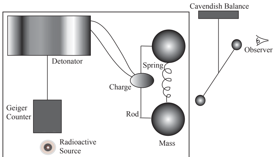
FIG. 5.1. Unruh's Schrödinger-Cavendish experiment: initial state
